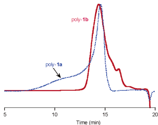
Figure 4. GPC chromatograms of poly- 1a and poly- 1b eluting with chloroform at a rate of 1.0 mL/min.
